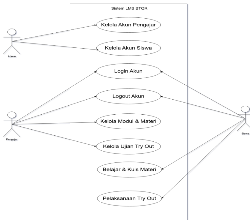
Gambar 3. 2 Usecase Diagram
